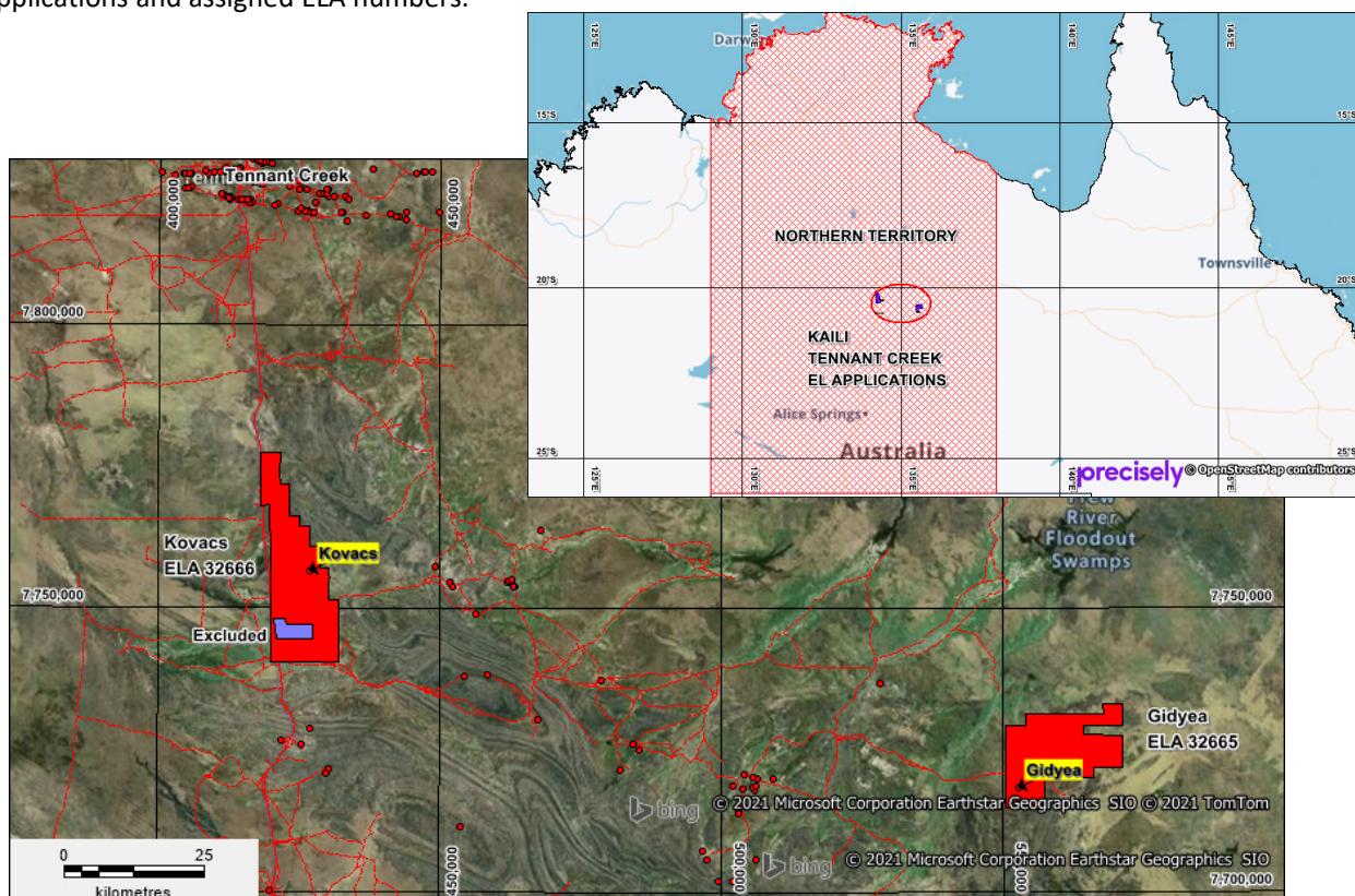
Figure 1: Regional Tenement Location SE of Tennant Creek – Kovacs and Gidyea
