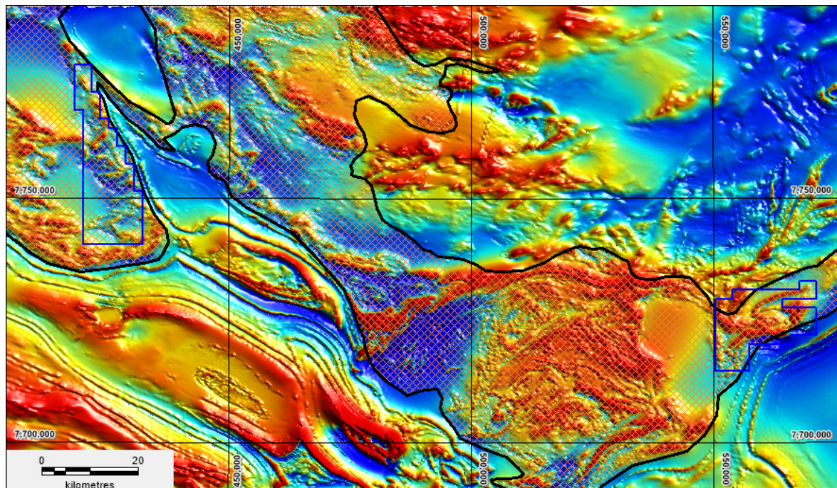
Figure 3: Gidyea (east) and Kovacs (west) are shown on regional TMI magnetics with the Warramunga Province shown as a light hatching over the magnetics.
