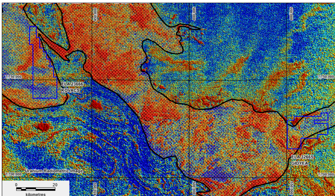
Figure 22: Gidyea and Kovac projects are shown on regional Uranium radiometrics with the Warramunga Province shown as a light hatching over the radiometrics.
