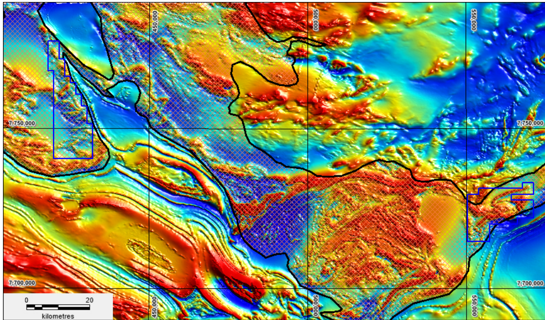
Figure 21: Gidyea (east) and Kovac (west) are shown on regional TMI magnetics with the Warramunga Province shown as a light hatching over the magnetics.
